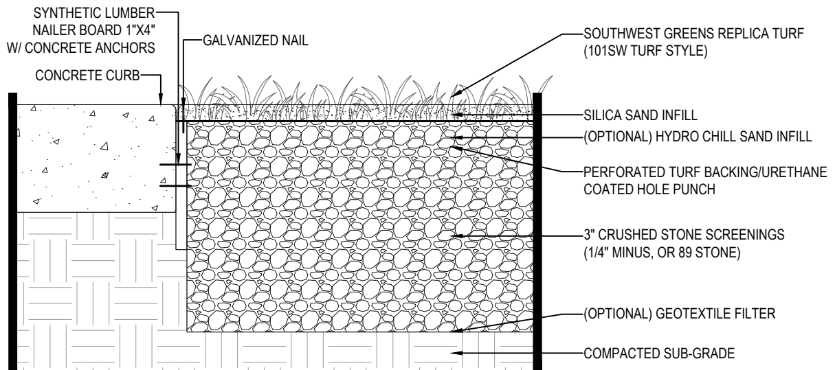
TYPICAL INSTALL CROSS SECTION
